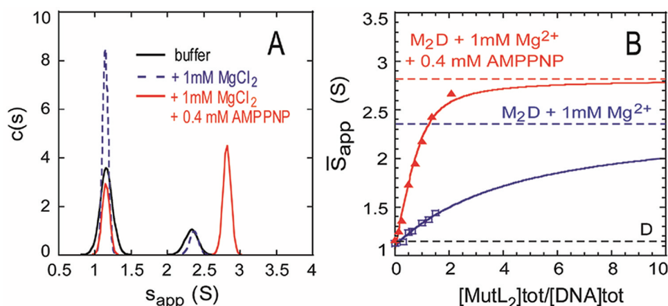
Figure 7. Sedimentation velocity study of binding of MutL dimer to a 3'-(dT 20 )-ds18 DNA. Experiments were performed at 25 °C using a total loading Cy3-DNA concentration of 1.4 μM as a function of MutL dimer concentration in M20/20 (buffer), with 1 mM MgCl 2 (+1 mM MgCl 2 ), or in M20/20 with 1 mM MgCl 2 and 0.4 mM AMPPNP (+1 mM MgCl 2 +0.4 mM AMPPNP). The DNA concentration profiles were recorded by monitoring the absorbance of Cy3 at 550 nm. (A) Sedimentation velocity experiments were performed at 42000 rpm. Representative c(s) distribution of Cy3-DNA in the presence of 1.4 μM MutL dimer ( M_2:D molar ratio of 1). Sedimentation coefficients are not corrected to the standard conditions. (B) Weight-average sedimentation coefficient as a function of the molar ratio of MutL dimer to DNA. The smooth curves are simulations using the best fit parameters derived from NLLS analysis of the data to a simple Langmuir isotherm and assuming that the plateau corresponds to the apparent s value for the MutL–DNA complex [+MgCl 2 , 2.36 \pm 0.02 S, apparent binding constant of (19 \pm 1.8) \times 10^4 M -1 ; +MgCl 2 +AMPPNP, 2.82 \pm 0.02 S, apparent binding constant of (38 \pm 2.5) \times 10^5 M -1 (eq 6 in Materials and Methods)].
