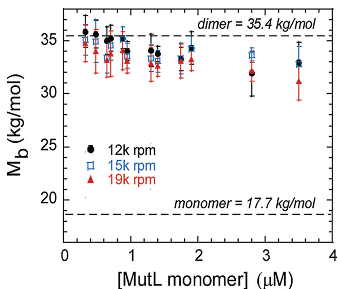
Figure 3. Weight-average buoyant molecular mass, \bar{M}_b , of MutL as a function of protein concentration. \bar{M}_b was determined with sedimentation equilibrium experiments performed at 5 °C at three rotor speeds (12000, 15000, and 19000 rpm) in buffer M [50 mM potassium phosphate (pH 7.4 at 25 °C), 50 mM KCl, 0.1 mM EDTA, and 1 mM 2-mercaptoethanol]. Each protein concentration distribution was fitted to a single-ideal species model [ n = 1 in eq 1 (Materials and Methods)]. Values of \bar{M}_b expected for the MutL monomer and dimer are indicated by dotted lines and calculated assuming monomer M = 67923.95 g/mol and \bar{v}_{5^\circ\text{C}} = 0.7329 mL/g, based on the amino acid sequence of MutL.
