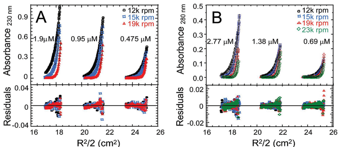
Figure 4. Sedimentation equilibrium data indicate that MutL is a stable dimer. Experiments were performed for three different MutL concentrations indicated on the plot (total monomer loading concentration) at three or four rotor speeds (12000, 15000, 19000, and 23000 rpm) at 5 °C in buffer M (A) or buffer M with 1 mM MgCl 2 and 35 μM AMPPNP (B). The smooth curves overlying the data are simulations using the best fit parameters resulting from a global NLLS fit of all data sets to a single-species model with residuals shown below the plots.
